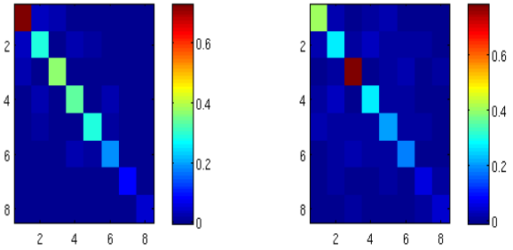
Figure 4: Frequency covariance matrices for state 'non-alpha' (left) and 'alpha' (right)
