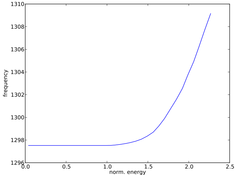
Figure 3: Frequency-energy plot of the first nonlinear mode
