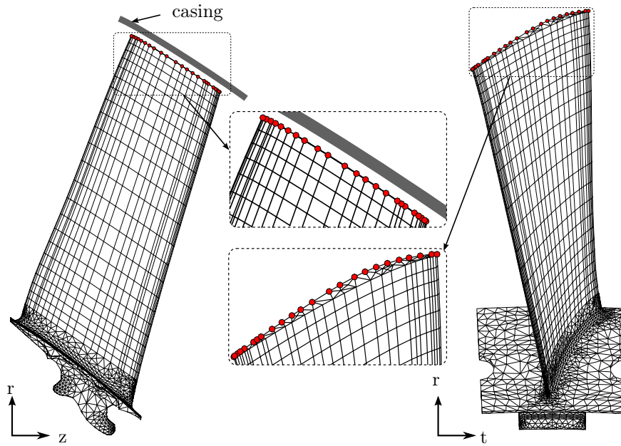
Figure 6: Blade model and details of the contact interface
