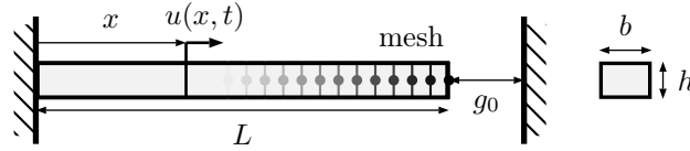
Figure 2: Thin rod in contact against a rigid foundation
