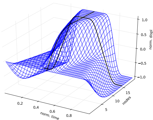
(c) displacement
