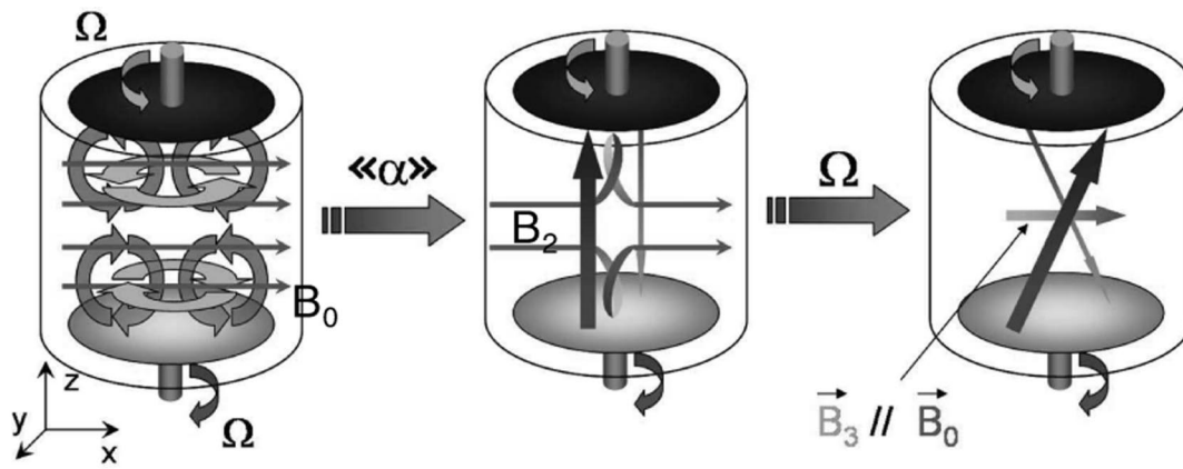
FIG. 10. “Alpha”-omega dynamo mechanism in the (DD) geometry: the applied transverse field (left) gives rise to the axial field displayed the middle figure—the “ \alpha ” step; via the \Omega effect, a third order induced field \mathbf{B}_3 is induced, parallel to \mathbf{B}_0 .
