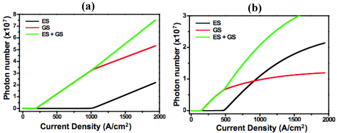
Figure 7. Calculated light-current characteristics of an 1.55 \mu\text{m} InAs/InP(311)B QD laser (a) without gain compression (b) including gain compression
