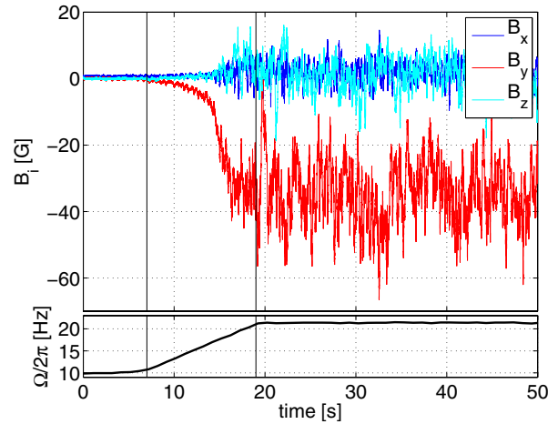
FIG. 2 (color online). Time recording at P1 of the components of the magnetic field when the rotation frequency \Omega/2\pi is increased as displayed by the ramp below ( R_m increases from 19 to 40).
