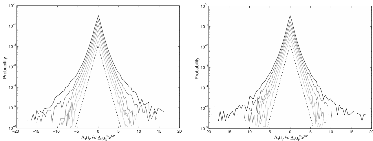
Figure 11. PDFs of the normalized increment \Delta_\tau u / \sigma_\tau for the two components of the velocity vector \mathbf{u} . The curves are shifted for clarity. From top to bottom: \tau = [0.125, 0.25, 0.5, 1, 2, 5] days. The dashed lines show an exponential decay and are for reference only.
