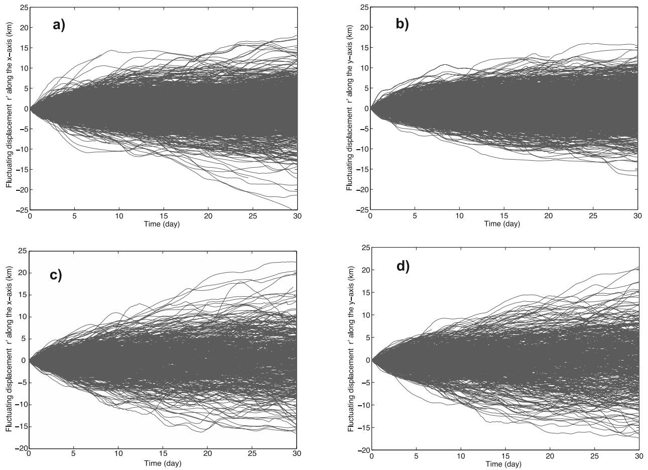
Figure 14. Particle displacements r'_x (along x ) and r'_y (along y ) caused by the fluctuating velocity field for (a and b) winter and (c and d) summer. The fluctuating displacements are calculated from buoy tracks for which the displacement associated with the mean flow is removed. After 30 days, fluctuating displacements are, on average, stronger in summer than in winter.
