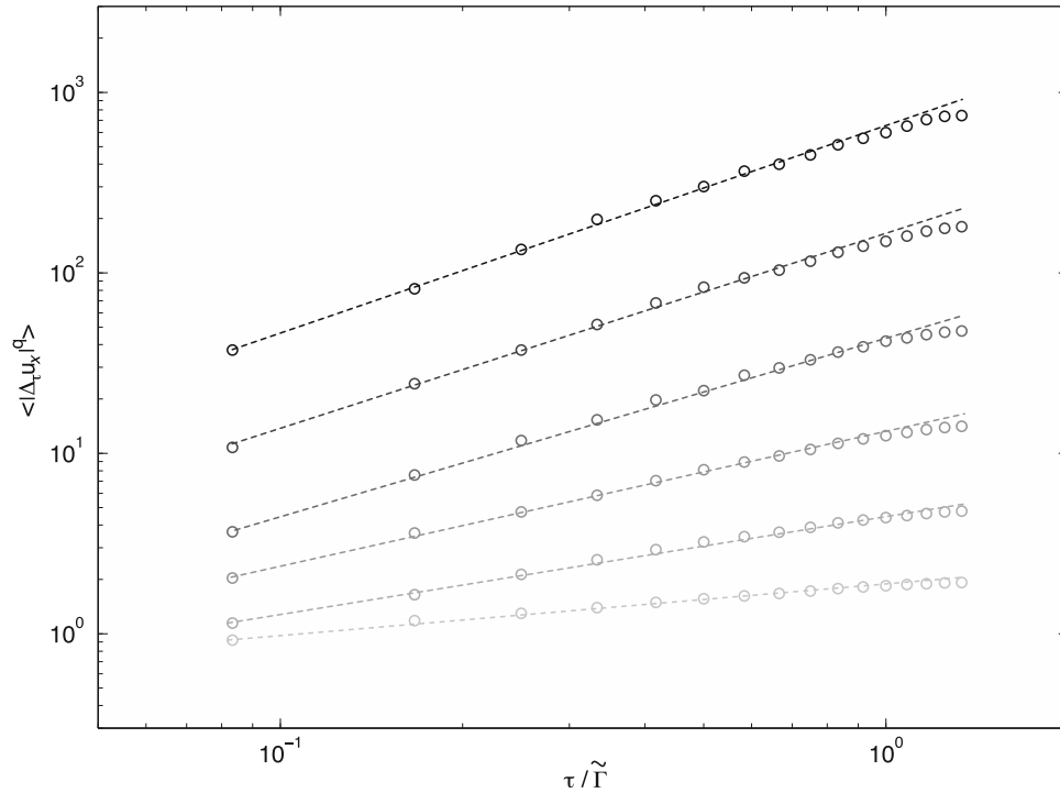
Figure 12. Lagrangian structure functions of the x component of the velocity for q = 0.5, 1, 1.5, 2, 2.5, and 3 for winter. The dashed lines are the least squares power law fits \langle |\Delta_\tau u|^q \rangle \sim \tau^{\zeta(q)} yielding the exponents \zeta(q) .
