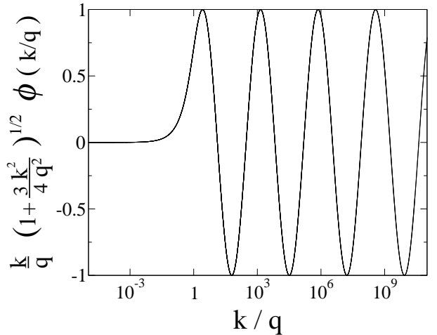
FIG. 1: Functions k/q \sqrt{1 + 3k^2/(4q^2)} \phi(k/q) obtained at unitarity ( |a| = \infty, R^* = 0 ) from Eq. (11) for the eight first trimers (including the ground state). The computation has been performed with the UV cut-off \Lambda_3 = 5 \times 10^2 \times \kappa^* . The function \sin \{ s_0 \operatorname{arcsinh}[k\sqrt{3}/(2q)] \} appearing in the exact solution Eq. (7) has been superimposed and is not distinguishable from the functions obtained by solving Eq. (11).
