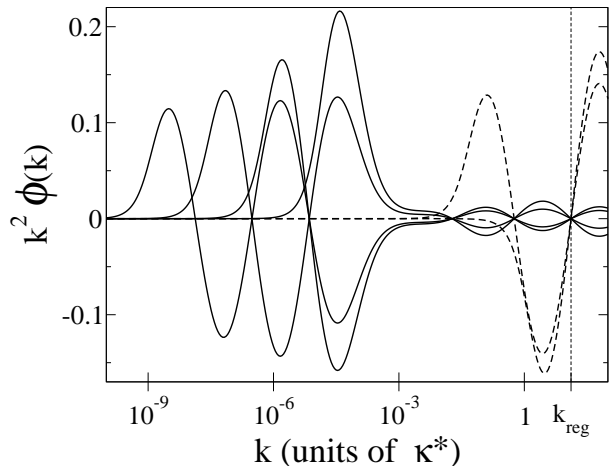
FIG. 3: Eigenfunctions k^2 \phi_n(k) for the deepest trimers states obtained after normalization of Eq. (11) for a_{\text{bg}} \kappa^* = -10^2 and R^* \kappa^* = 10^4 . Solid lines: eigenstates with a binding wavenumber given approximately by the spectrum of a narrow resonance [ q_p = \kappa^{*'} \exp(p\pi/s_0) ]. Dashed lines: eigenstates with a binding wavenumber given approximately by the spectrum of a broad resonance [ q_n = \kappa^* \exp(n\pi/s_0) ]. Dotted vertical line: position of the node imposed by Eq. (10).
