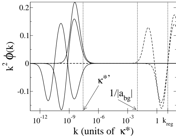
FIG. 4: Same as Fig. (3), but for a_{\text{bg}}\kappa^* = -10^2 and R^*\kappa^* = 10^8 . In this regime, characterized by the inequality R^* \gg |a_{\text{bg}}| , there is a clear separation of scale for the two type of eigenstates: the deepest one of the 'broad type' are located in the momentum region k \gtrsim 1/|a_{\text{bg}}| , those of the 'narrow type' are located in the momentum region k \lesssim \kappa^* .
