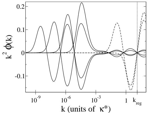
FIG. 3: Eigenfunctions k^2 \phi_n(k) for the deepest trimers states obtained after normalization of Eq. (11) for a_{\text{bg}} \kappa^* = -10^2 and R^* \kappa^* = 10^4 . Solid lines: eigenstates with a binding wavenumber given approximately by the spectrum of a narrow resonance [ q_p = \kappa^{*' } \exp(p\pi/s_0) ]. Dashed lines: eigenstates with a binding wavenumber given approximately by the spectrum of a broad resonance [ q_n = \kappa^* \exp(n\pi/s_0) ]. Dotted vertical line: position of the node imposed by Eq. (10).
