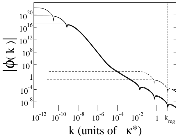
FIG. 5: Absolute value of the eigenfunctions |\phi(k)| in Fig. (4) ( a_{\text{bg}}\kappa^* = -10^2 , R^*\kappa^* = 10^8 ) in logarithmic scale. The figure, shows that even in this regime where 'broad type' and 'narrow type' eigenfunctions are well separated, eigenfunctions share the same 0 at k = k_{\text{reg}} . 'Narrow type' eigenstates experience a k^{-4} power law in the region 1 \ll kR^* \ll \sqrt{\frac{R^*}{|a_{\text{bg}}|}} .
