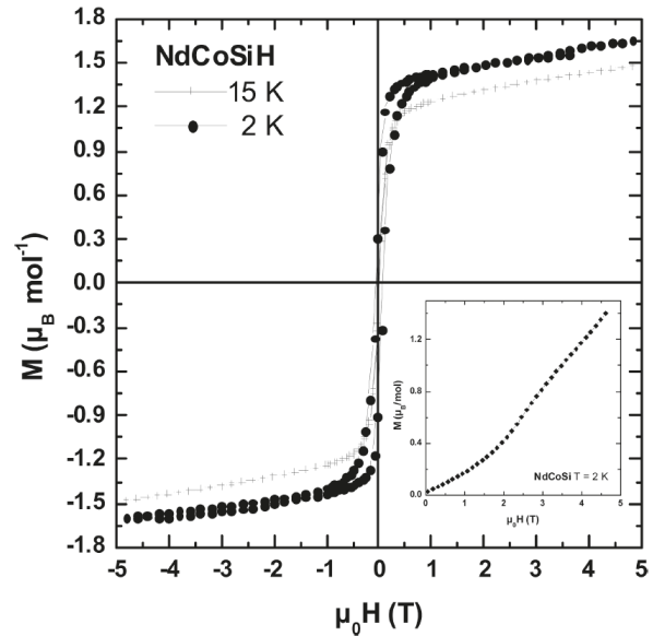
Figure 2. Field dependence at 2 and 15 K of the magnetization M for NdCoSiH. The inset presents the curve M versus \mu_0 H for NdCoSi cooled at 2 K.
