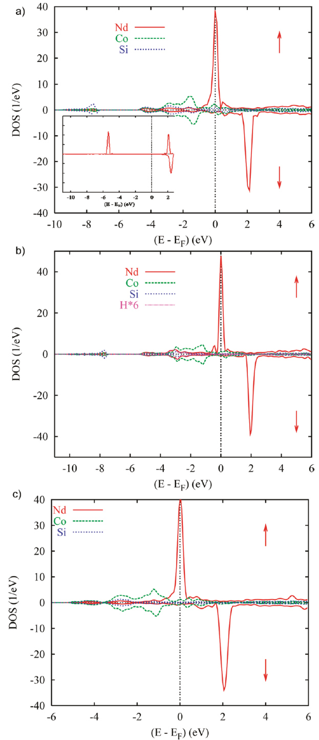
Figure 7. Site and spin projected density of states (PDOS) for a ferromagnetic configuration of (a) NdCoSi (the inset shows the change of Nd PDOS from GGA+ U calculations), (b) NdCoSiH (H PDOS were artificially multiplied by 6 for sake of clear presentation), and (c) NdCoSi expanded.
