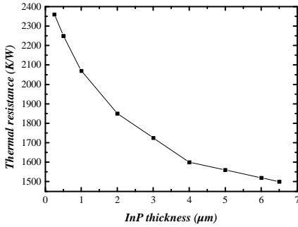
Figure 4. Electrical VCSEL thermal resistance as a function of InP thickness.
