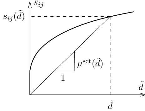
Figure 2: Secant modulus formulation of nonlinear incompressible isotropic fluid.
