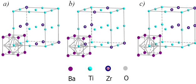
FIG. 1: (Color online) Arrangements of the 20 Ti- and 7 Zr-atoms in the \text{BaTi}_{0.74}\text{Zr}_{0.26}\text{O}_3 supercells used for our calculations. Only one of the 27 perovskite unit cells is fully represented to facilitate the visualization of the supercells.
