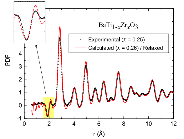
FIG. 2: (Color online) Experimental pair distribution function of \text{BaTi}_{0.75}\text{Zr}_{0.25}\text{O}_3 at 300 K (open circles) 14 , compared with the PDF calculated from the three relaxed supercells of \text{BaTi}_{0.74}\text{Zr}_{0.26}\text{O}_3 (line).
