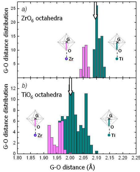
FIG. 3: (Color online) Distribution of the distance between the center of mass of oxygens (denoted G) and the oxygens calculated from the three relaxed supercells of \text{BaTi}_{0.74}\text{Zr}_{0.26}\text{O}_3 : (a) for the \text{Zr-O}_6 octahedra, and (b) for the \text{Ti-O}_6 octahedra. The G-O segments that are directed toward Zr and Ti neighbors are represented in light magenta and dark green, respectively. The arrows mark the mean G-O distances calculated for the \text{Zr-O}_6 and \text{Ti-O}_6 octahedra.
