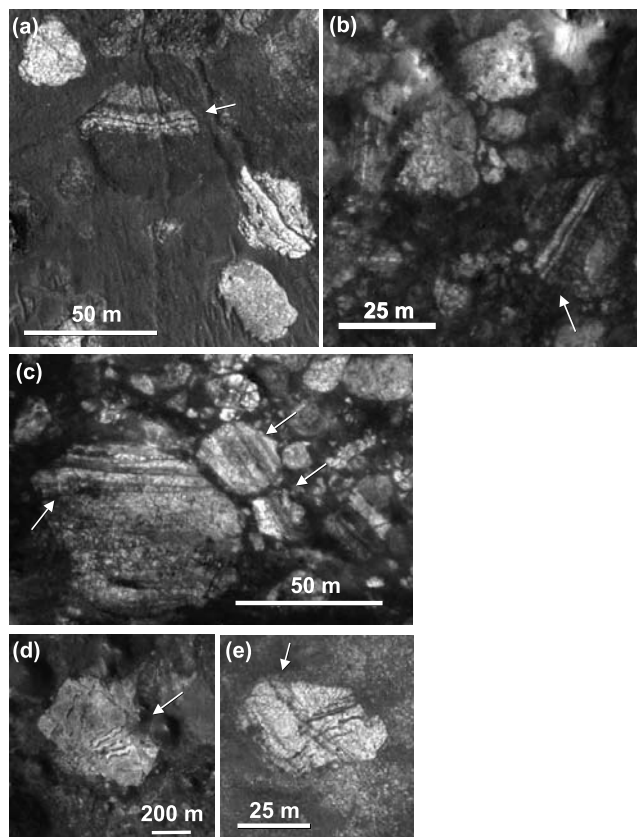
Figure 14. Breccia blocks with meter-scale layering within basement rocks in Nili Fossae. HiRISE images are from subsets of (a) PSP_002176_2075, (b) PSP_007569_2020, (c) PSP_006923_1995, (d) PSP_3086_2015, and (e) PSP_2176_2075.
