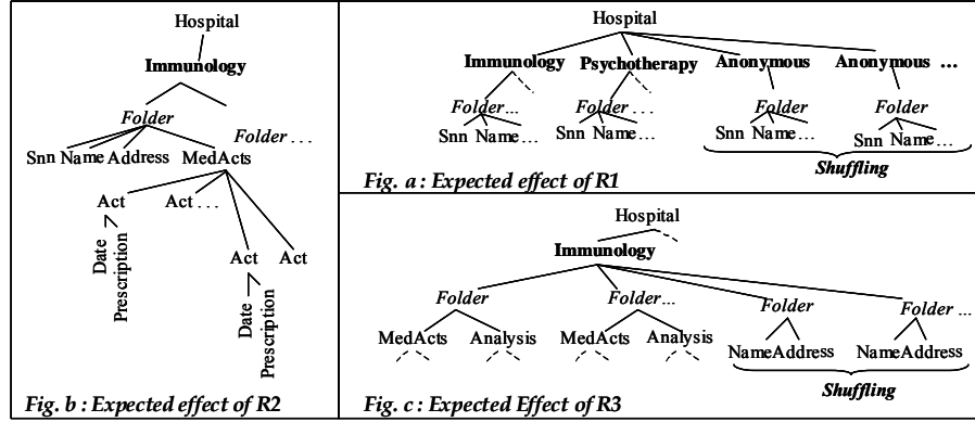
Figure 2: Authorized views.
