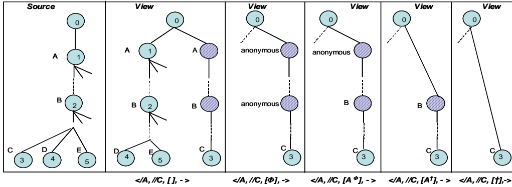
Figure 3: Path-Visibility example.
