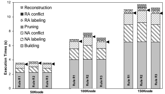
Figure 6: Impact of RA on the motivating example.
