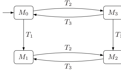
Figure 2. Graph of reachable markings
