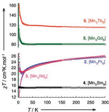
Figure 5. Temperature dependence of the \chi T products for 2–6 at 1000 Oe (with \chi = M/H ). The solid lines are the best fit obtained using a Curie–Weiss law above 30 K for 2 and 3 and down to 1.8 K for 5 and 6 . The values of the obtained Curie and Weiss constants are given in Table 4. It is worth noting that a simple Curie behavior is seen for 4 .
