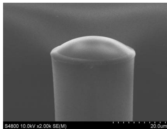
Fig. 11. SEM image of a microlens with a diameter of 30\ \mu\text{m} deposited on a cylindrical pedestal.
