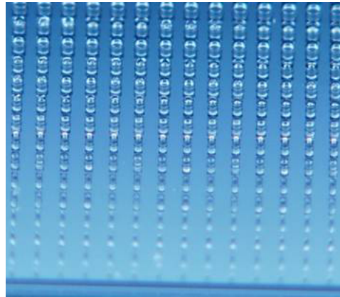
Fig. 12. Microscope image of an array of cylindrical pedestals of various diameters [30-140 \mu\text{m} ] with microlenses deposited on their surfaces.
