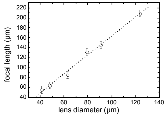
Fig.8. Evolution of focal length as a function of lens diameter
