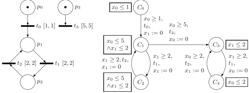
Fig. 3. Looping with domain union
