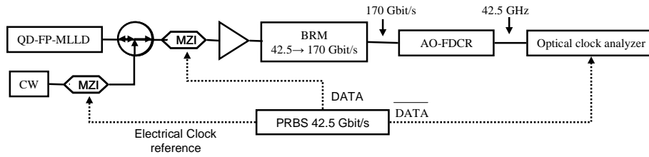
Fig.3. AO-FDCR experimental setup
