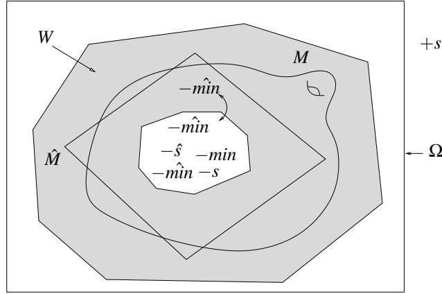
Figure 7: Condition 2'. and 4. are necessary.
