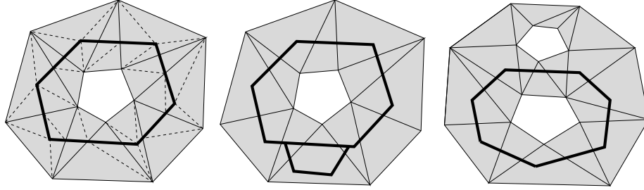
Figure 2: The grey complex L on the left collapses to the bold curve K (dashed edges represent the subdivision L' ). This is not true for the two other complexes.
