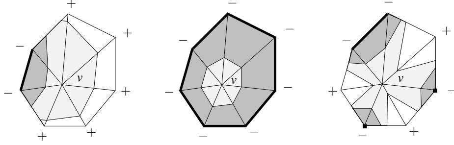
Figure 4: Morse theory for PL functions in 2D. Plus and minus signs indicate whether neighbors of v are larger or smaller than v . Lower links are displayed in bold, sets \hat{f}^{-1}(]-\infty, f(v) - \epsilon]) in grey, and sets \hat{f}^{-1}([f(v) - \epsilon, f(v) + \epsilon]) in light grey.
