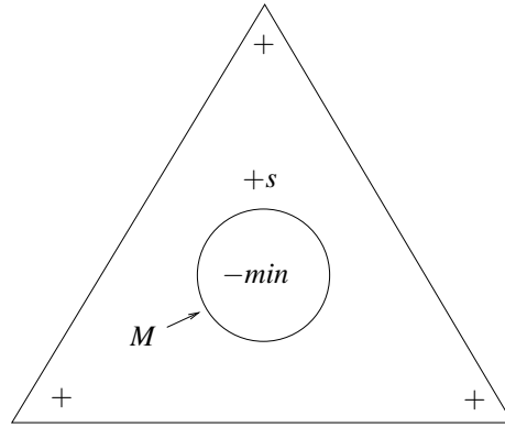
Figure 5: Condition 0. is necessary.
