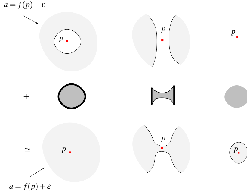
Figure 3: Smooth Morse theory in 2D.
