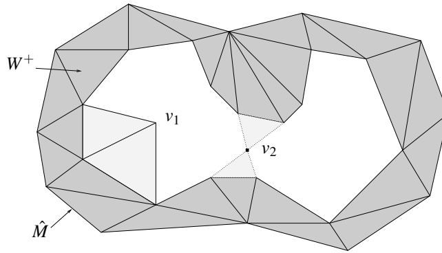
Figure 9: Construction of W^+ : lower stars of regular vertices (such as v_1 ) are added one by one. Lower stars of critical vertices ( v_2 ) are discarded.
