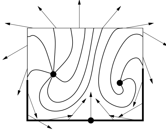
Figure 12: An index 2 vector field V on a square C represented by a few flow lines. \partial_- C is in bold. The dot on \partial_- C represents the unique zero of \partial_- V , which has index -1 .
