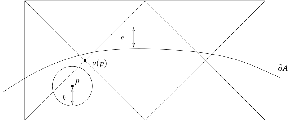
Figure 11: Proof of lemma 11.
