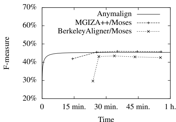
Figure 3: Comparison of the outputs of the three word aligners against a reference bilingual lexicon on the French-Spanish task.
