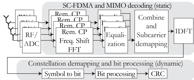
Figure 2. The uplink decoding static and dynamic parts.
