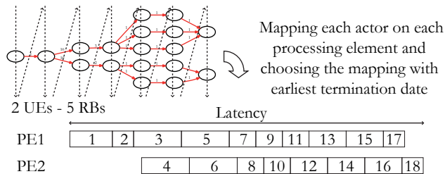
Figure 9. Example of the list scheduling of HDAG actors.
