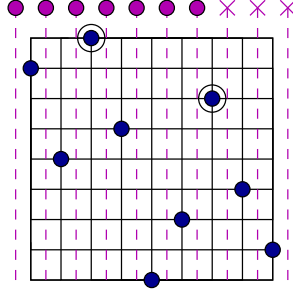
FIGURE 1. The permutation \tau = 8\ 5\ 9\ 6\ 1\ 3\ 7\ 4\ 2 \in \mathfrak{S}_9^{(3)} . One has a_1(\tau) = 1 , a_2(\tau) = 3 , a_3(\tau) = 7 . There are 7 admissible ways to insert the value 10. Inserting 10 to the right of \tau(7) would create an occurrence of 1234.
