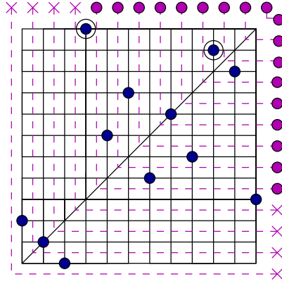
FIGURE 2. The involution \tau = 3\ 2\ 1\ 12\ 7\ 9\ 5\ 8\ 6\ 11\ 10\ 4 \in \mathfrak{J}_{12}^{(5)} . One has a_1(\tau) = 3 , a_2(\tau) = 9 . There are 9 admissible ways to insert a 2-cycle.
