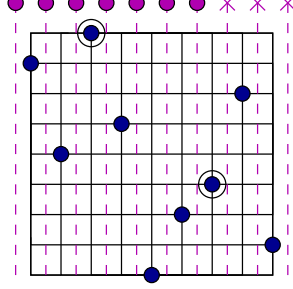
FIGURE 1. The permutation \tau = 8\ 5\ 9\ 6\ 1\ 3\ 4\ 7\ 2 \in \mathfrak{S}_9^{(3)} . One has a_1(\tau) = 1 , a_2(\tau) = 3 , a_3(\tau) = 7 . There are 7 admissible ways to insert the value 10. Inserting 10 to the right of \tau(7) would create an occurrence of 1234.
