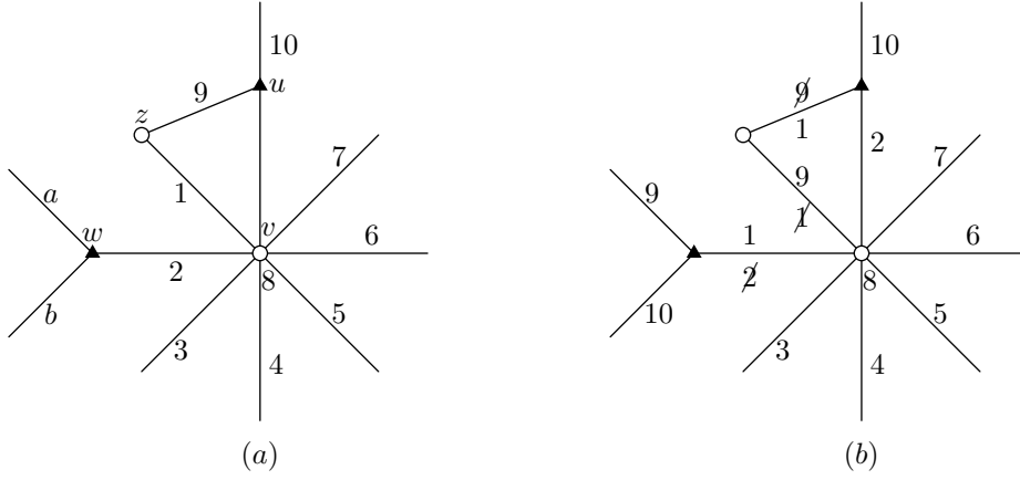
Figure 4: Coloring and recoloring for the proof of Lemma 5.
