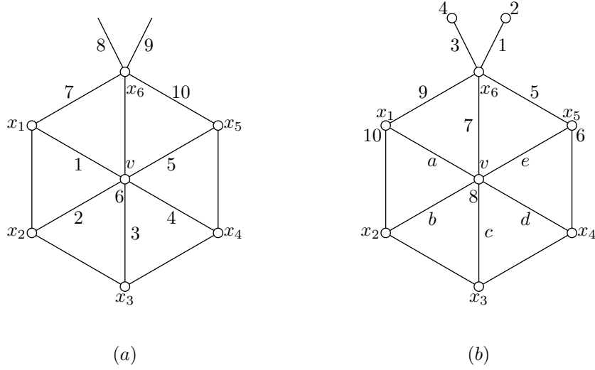
Figure 8: Proof of Lemma 10: (a) coloring of G - vx_6 , (b) partial coloring of G in which x_6 is not colored.
