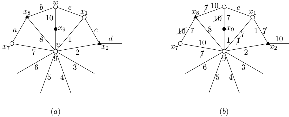
Figure 9: Precoloring and recoloring for the proof of Lemma 11.
