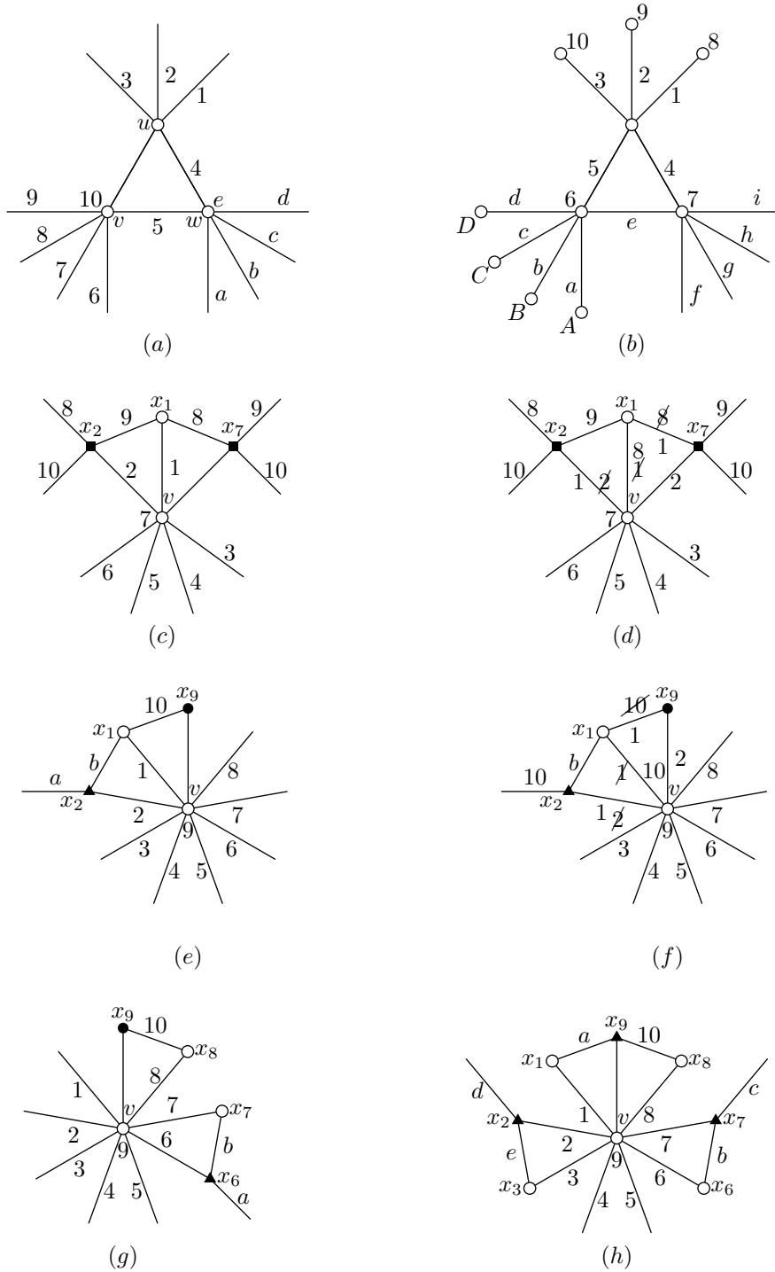
Figure 3: Configurations for the proofs of Lemmas 3 and 4.
