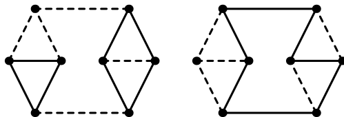
Figure 10: Spanning subgraphs of the graph H_3 showing that every vertex of H_3 is trimatched (symmetric cases are omitted). The edges contained in the subgraphs are dashed.
