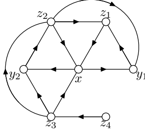
Figure 3: Configuration obtained when \varphi(x) = 2 .
