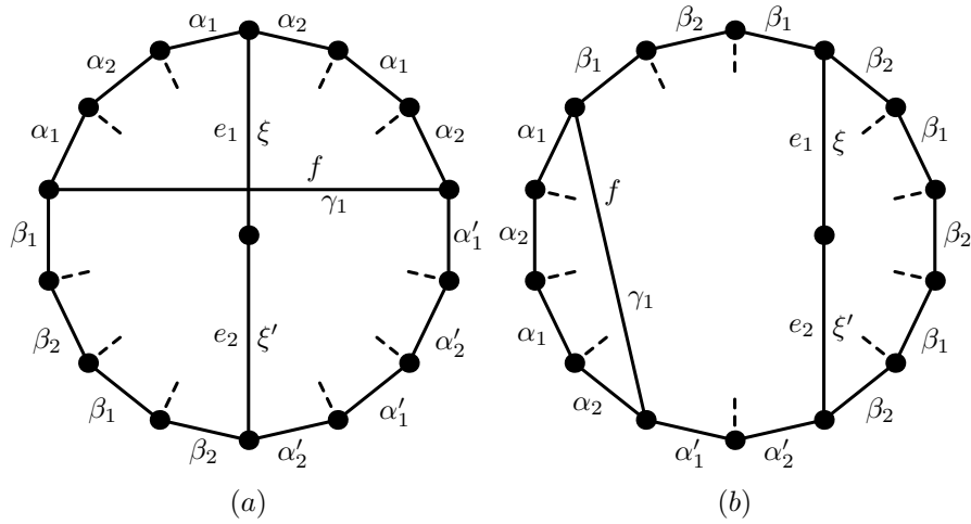
Figure 16: The colourings of G_0 constructed in the proof of Lemma 13 in the case where the cycle C_e is even and (a) the chords e and f cross, (b) the chords e and f do not cross. The dashed chords are labelled with \xi .
