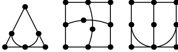
Figure 2: The three forbidden configurations for affine Steiner triple systems: the configurations C_{16} , C_S^1 and C_S^2 (from left to right).
