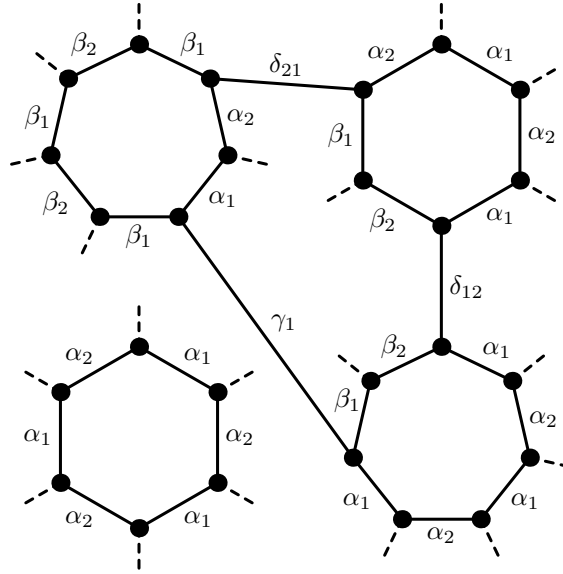
Figure 12: The colouring constructed in the proof of Theorem 8. The edges of M \setminus (T_1 \cup T_2) are drawn as dashed and coloured with the point \xi .
