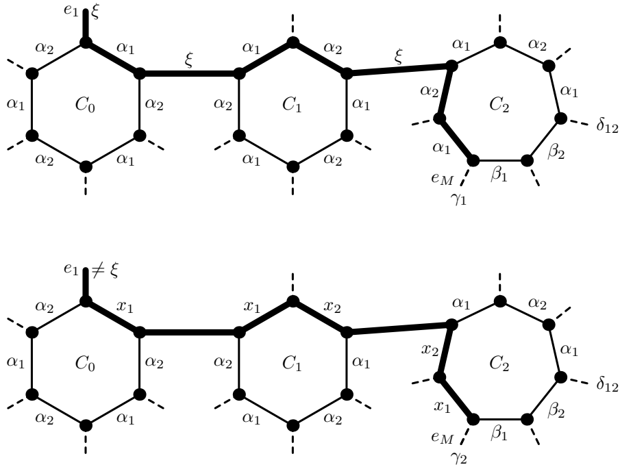
Figure 14: The modification of the colouring performed in the proof of Lemma 12—the original colouring is in the top and the modified in the bottom of the figure. The edges of the path P are drawn solid bold.
