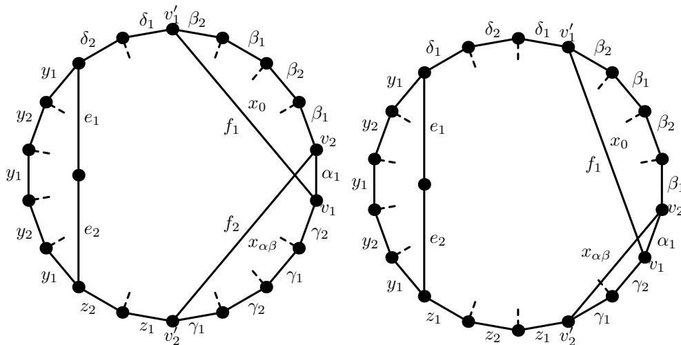
Figure 19: The colourings of G_0 constructed in the proof of Lemma 14 in the case where there is no chord crossing e . The dashed chords are labelled with \xi .
