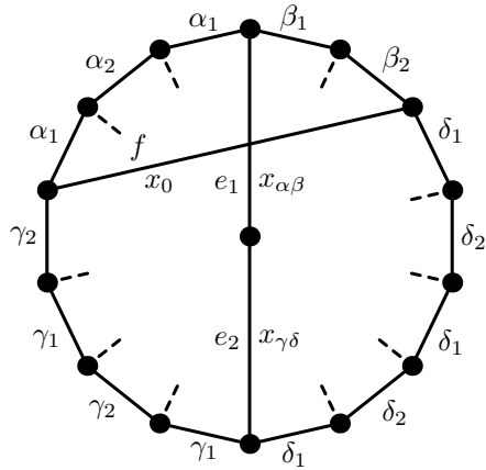
Figure 18: The colouring of G_0 constructed in the proof of Lemma 14 in the case where there is a chord crossing e . The dashed chords are labelled with \xi .
