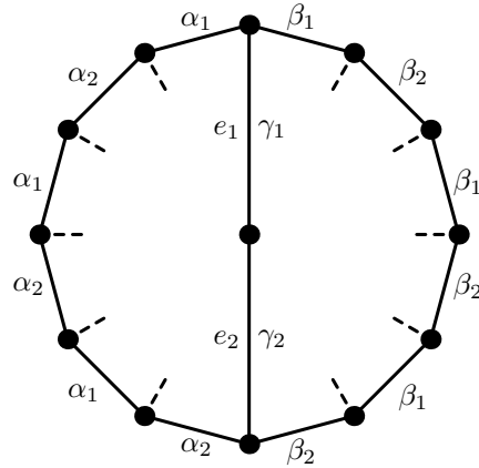
Figure 15: The colouring of G_0 constructed in the proof of Lemma 13 in the case where the cycle C_e is odd in G . The dashed chords are labelled with \xi .
