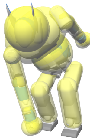
Fig. 8. Simplified model of the robot for posture optimization
