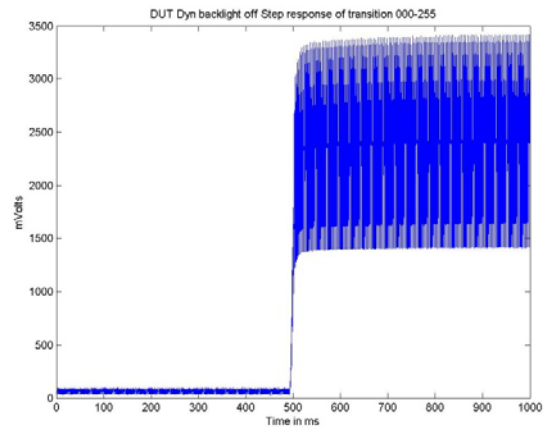
Figure 4: The raw response time data from the transition 0 to 255, when the dynamic backlight is off
