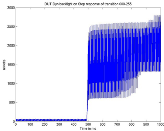
Figure 2: The raw response time data from the transition 0 to 255, when the dynamic backlight is on
