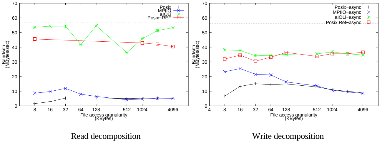
Figure 5: 1 IOR - Validation of aggregation mechanisms inside aIOLi
