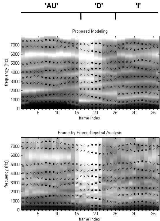
Figure 2. Spectrograms of the sequential phonemes 'AU'- 'D'-'I' from a French phrase. Peak locations calculated from our proposed analysis are indicated in both plots by black circles (filled indicate stable center frames).
