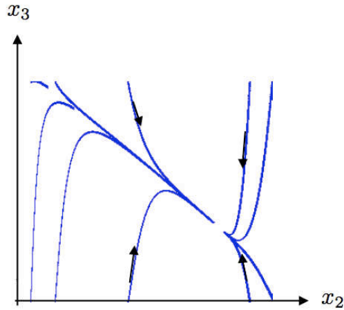
FIGURE 5. On this picture we have represented the projection of simulations of the the complete system (6) on the plane (x_2, x_3) . The variables (s_1, x_1) (not represented) present rapid oscillations while (x_2, x_3) evolves slowly. One sees that all the trajectories seem to converge to an equilibrium. Compare to the “theoretical” picture on Fig 8.
