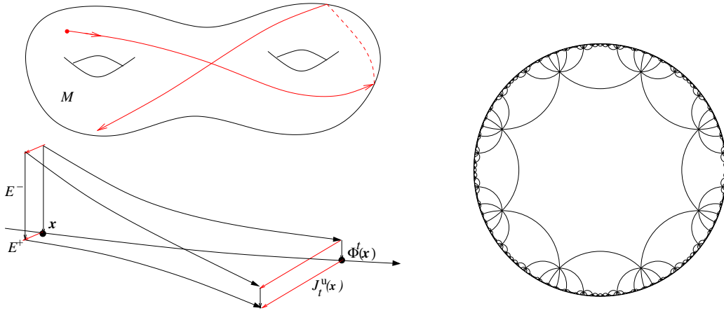
Figure 3: Top left: geodesic flow on a surface of negative curvature (such a surface has a genus \geq 2 ). Right: fundamental domain for an “octagon” surface \Gamma \backslash \mathbb{H} of constant negative curvature (the figure is due to C. McMullen) Bottom left: a phase space trajectory and two nearby trajectories approaching it in the future or past. The stable/unstable directions at \mathbf{x} and \Phi^t(\mathbf{x}) are shown. The red lines feature the expansion along the unstable direction, measured by the unstable Jacobian J_t^u(\mathbf{x}) = \det(d\Phi^t|_{E_{\mathbf{x}}^+}) .
