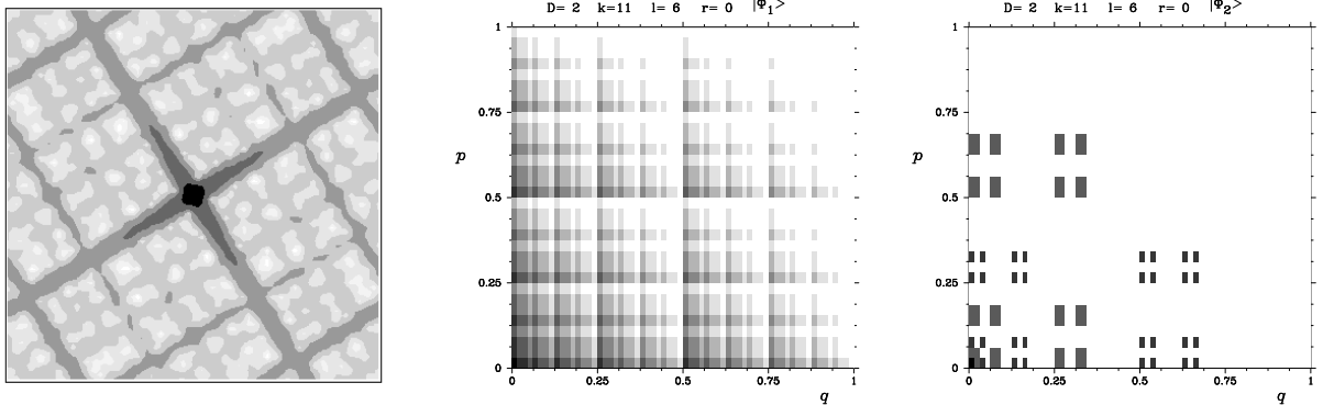
FIGURE 9. Left: Husimi density of an eigenstate of U_N(S_{cat}) , strongly scarred at the origin (from [42]). Notice the hyperbolic structure around the fixed point. Center, right: two eigenstates of the Walsh-quantized baker's map (plotted using a “Walsh-Husimi measure”); the corresponding semiclassical measures are fractal (from [2]).
