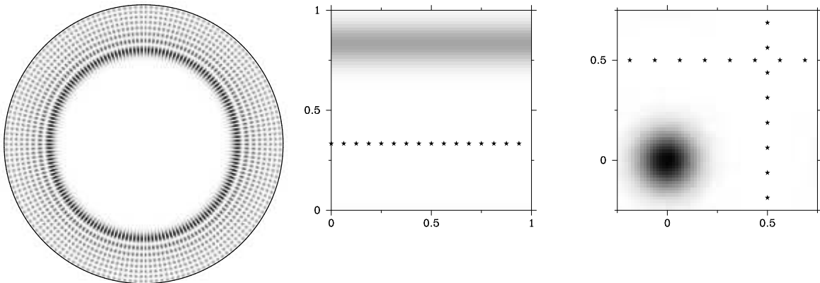
FIGURE 7. Left: one eigenmode of the circle billiard, microlocalized on a certain torus T_{\bar{I}} ( I_1, I_2 can be taken to be the energy and the angular momentum). Center: Husimi density of a simple Lagrangian state on \mathbb{T}^2 , namely a momentum eigenstate microlocalized on the lagrangian \{\xi = \xi_0\} . Right: Husimi density of the Gaussian wavepacket (21). Stars denote the zeros of the Husimi density. (reprinted from [79])
