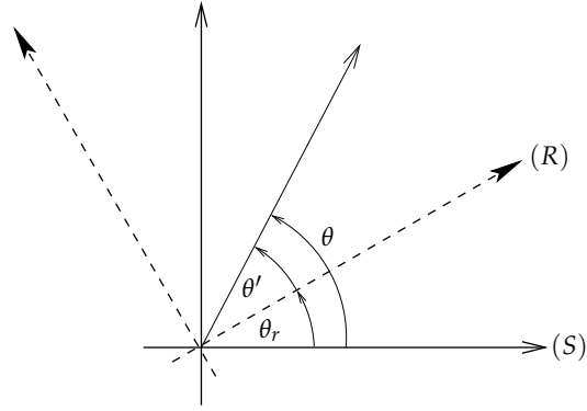
Fig. 1. Stator (S) and rotor (R) reference frame
