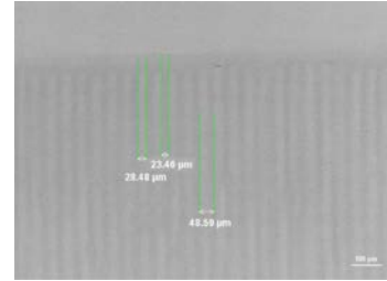
Figure 3. Optical verification of the poling efficiency, case of a 50 μm period device, evidence of contrast changes between Z+ (native polarization) and Z- (switched polarization) domains. The evidence of contrast modification in the vicinity of the poled domain strip edge (the whole plate is Z+ oriented, the poled strips are Z- oriented) may be due to diffusion effects
