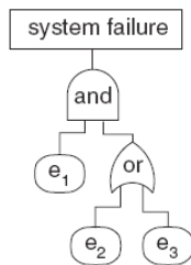
Figure 5: An example of a fault-tree of a three components system
