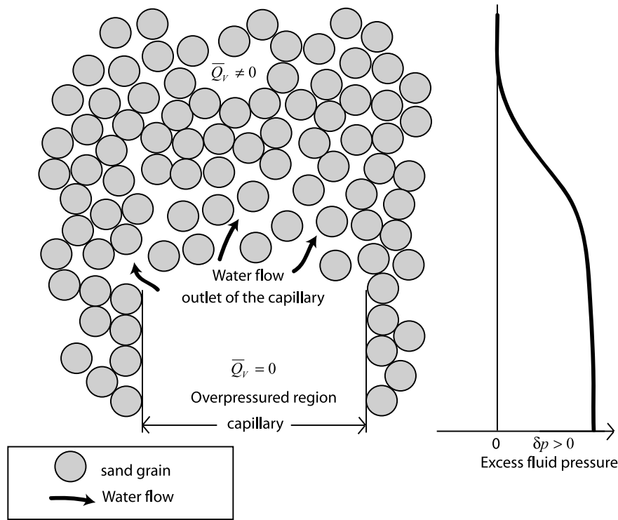
Figure 11. The boundary between the inlet / outlet of the capillary and the surrounding sand is characterized by a drop in the charge density per unit pore volume \bar{Q}_v . The resulting dipolar momentum vector \mathbf{P} is oriented downward. Its position is likely to be located slightly above the capillary outlet. Its strength is expected to decrease over time because of the decrease of the fluid pressure over time due to the diffusion of the pressure field around the outlet of the capillary.
