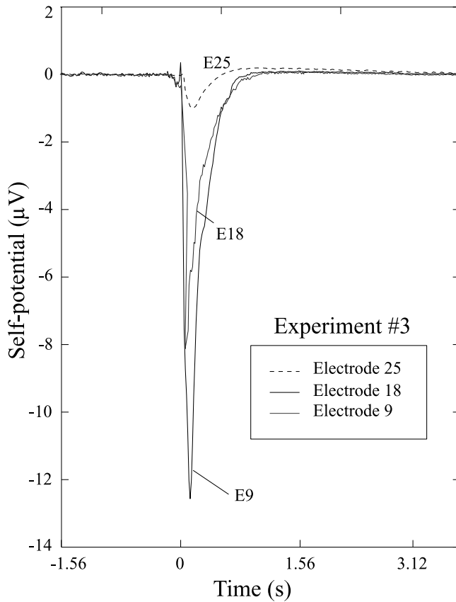
Figure 8. Injection experiment (Experiment #3). Time variation of the self-potential of three selected electrodes.
