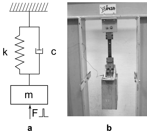
Fig. 10. Experimental set-up for the local belt characteristics identification.
