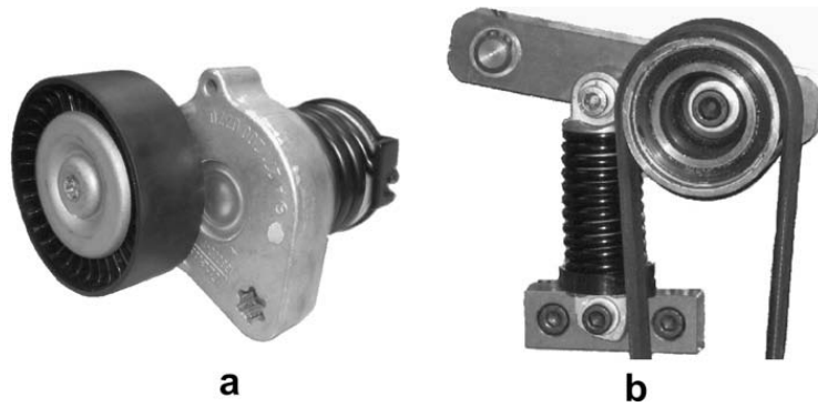
Fig. 1. Tensioner types: dry friction (a) and hydraulic (b).
