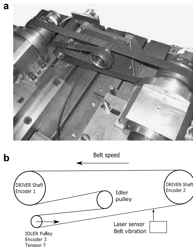
Fig. 2. Multi ribbed belt generic transmission set-up.
