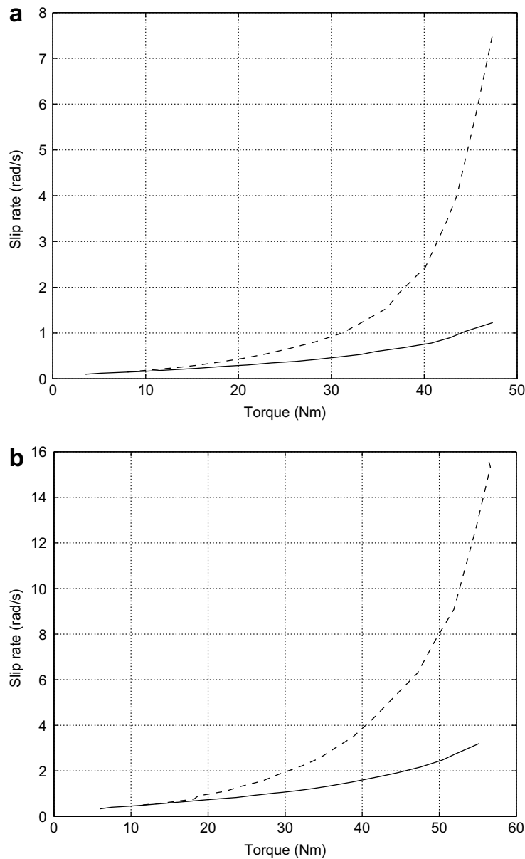
Fig. 8. Slip rate, pulley 4 fixed, initial tension 111 N(-) and 274 N (-), driving speed (a) 280 rpm and (b) 840 rpm.
