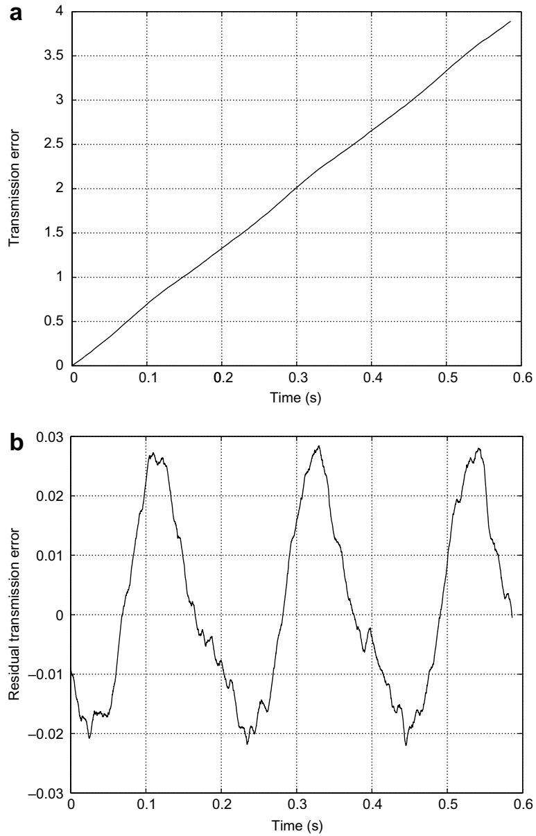
Fig. 6. Total (a) and residual (b) transmission error vs. time.
