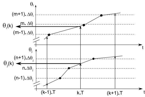
Fig. 5. Time re-sampling of encoder signals.
