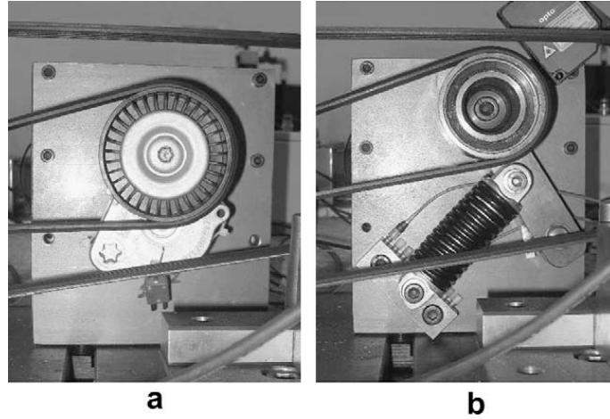
Fig. 3. Dry friction (a) and hydraulic (b) tensioner assemblies on the transmission.
