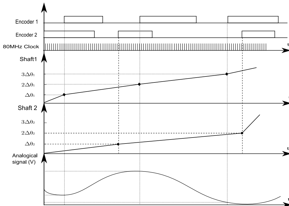
Fig. 4. Pulley angular rotations measurement principle.
