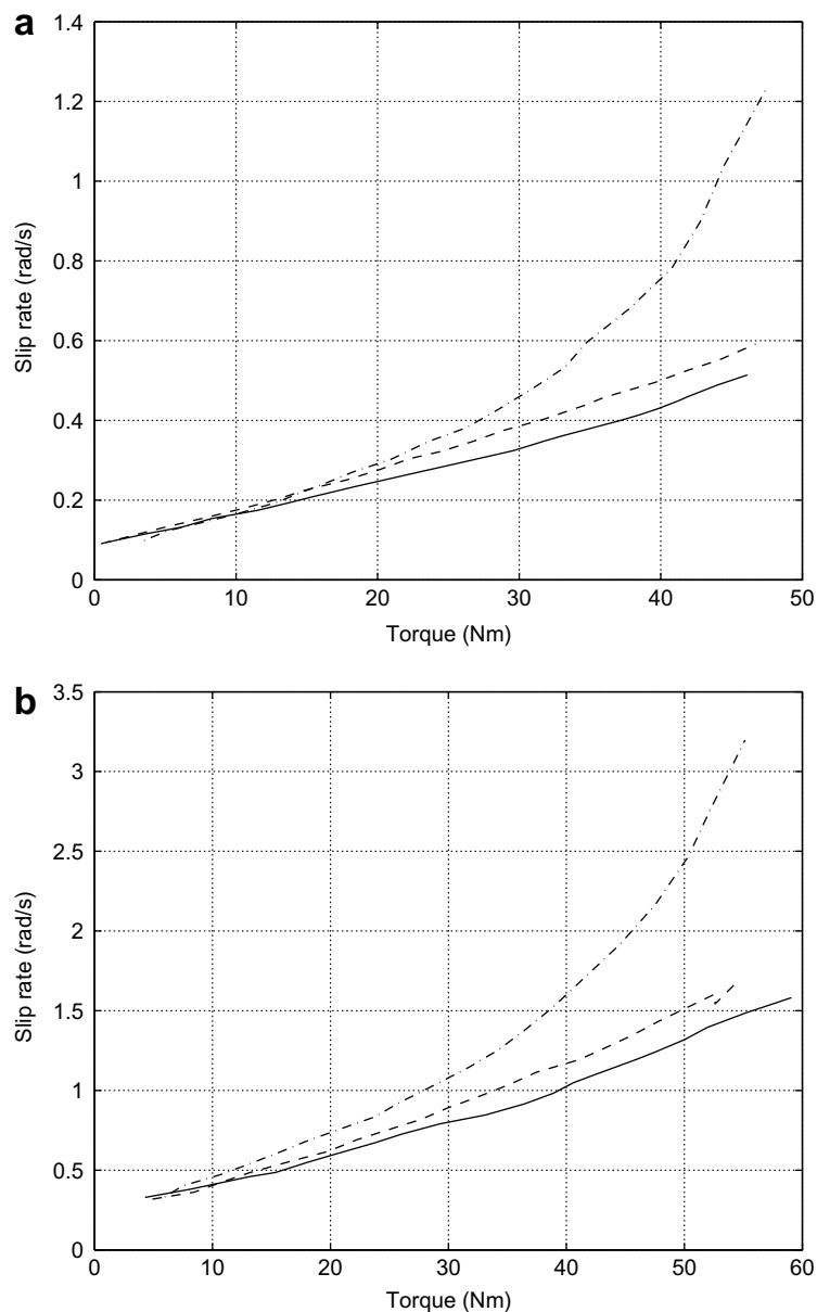
Fig. 7. Slip rate when pulley 4 is an idler (-·-), dry friction (- -) or hydraulic (-) tensioner, at driving speeds (a) 280 rpm and (b) 840 rpm.
