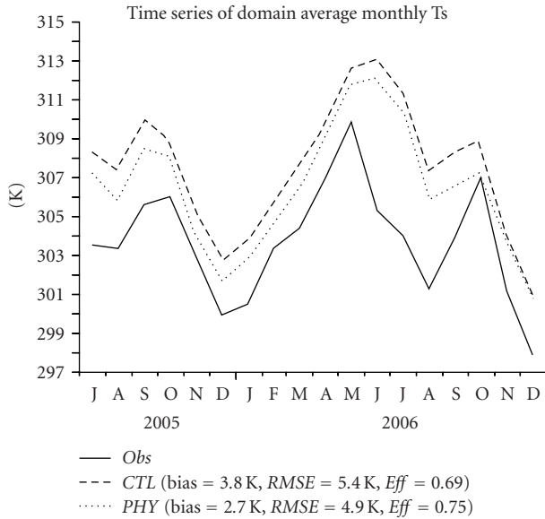
FIGURE 4: Comparison between the simulated and MSG/SEVIRI estimated monthly surfaces temperatures over Dantiandou Kori. The Bias, RMSE, and Efficiency ( Eff ) statistics calculated at a 3-hour time step are also given.
