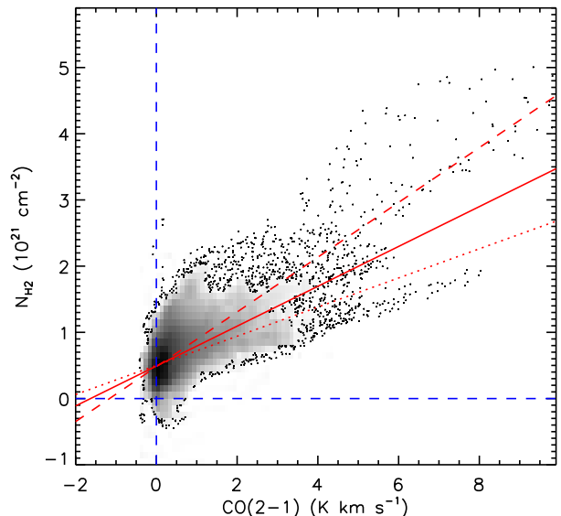
Fig. 5. Scatter plot of H_2 column density as derived from the dust emission and the CO(2-1) intensity. The solid red line is a fit to the entire dataset and corresponds to a N(H_2)/I_{\text{CO}(2-1)} value of 3 \times 10^{20} \text{ H}_2 per \text{K km s}^{-1} with an offset as described in the text. A radial variation is present: fitting within 2 kpc yields a N(H_2)/I_{\text{CO}(2-1)} value of 2.2 \times 10^{20} \text{ H}_2 per \text{K km s}^{-1} and 4.1 \times 10^{20} \text{ H}_2 per \text{K km s}^{-1} beyond 2 kpc (dotted and dashed lines, respectively).
