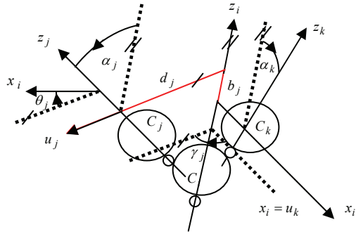
Figure 1. Geometric parameters
