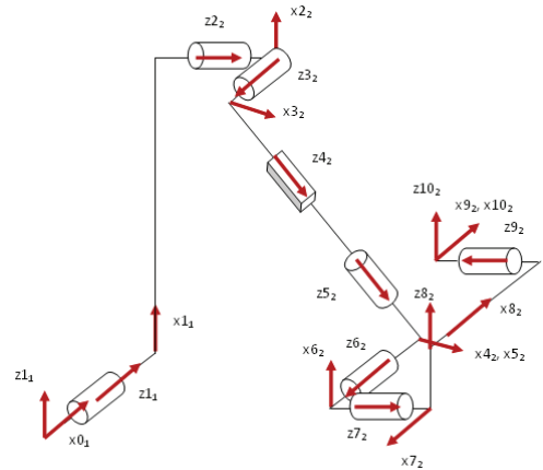
Figure 5. Description of loop LP2
