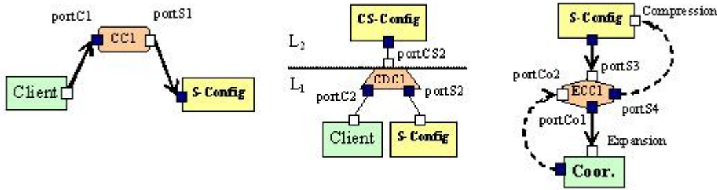
Figure 3: CC, CDC and ECC connector types in client-server architecture
