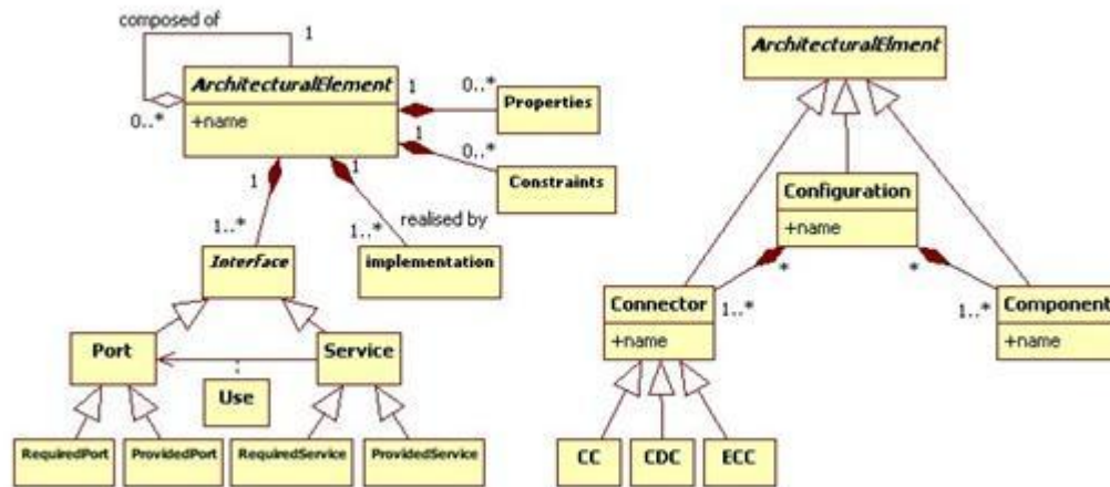
Figure 1: Architectural elements and their structure in C3
