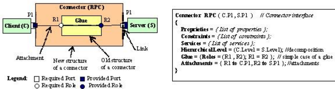
Figure 2: RPC connector structure and signature in C3
