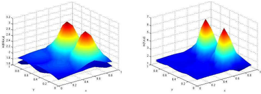
(a) Densities at instant t = 0.9 (b) Densities at instant T=1
