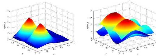
(a) Densities at instant t = 0.1 (b) Densities at instant t = 0.4
