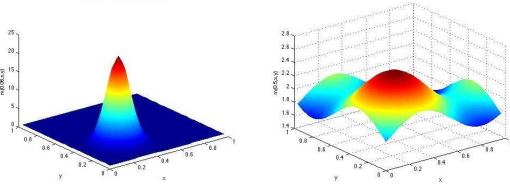
(a) Density at instant t = 0.06 (b) Density at instant t = 0.5
