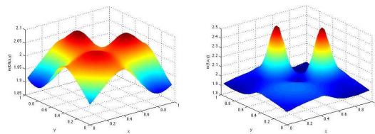
(a) Density at instant t = 0.9 (b) Density at instant T = 1
