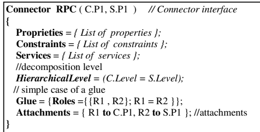
Figure 6.b. Connector description in C3
