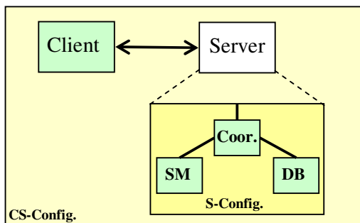
Figure 5. Client-Server Architecture
