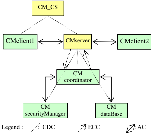
Figure 11. Physique architecture of client-server application
