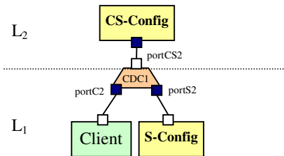
Figure 8.b. Possible links of CDC1 connector
