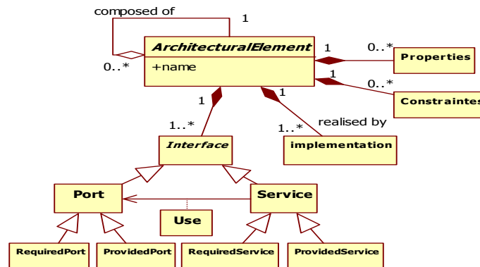
Figure 2. Structure of an architectural element in C3
