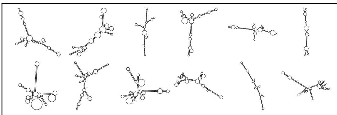
Loops model \mathcal{M}_L : Constrained hairpins and multiple loops.
