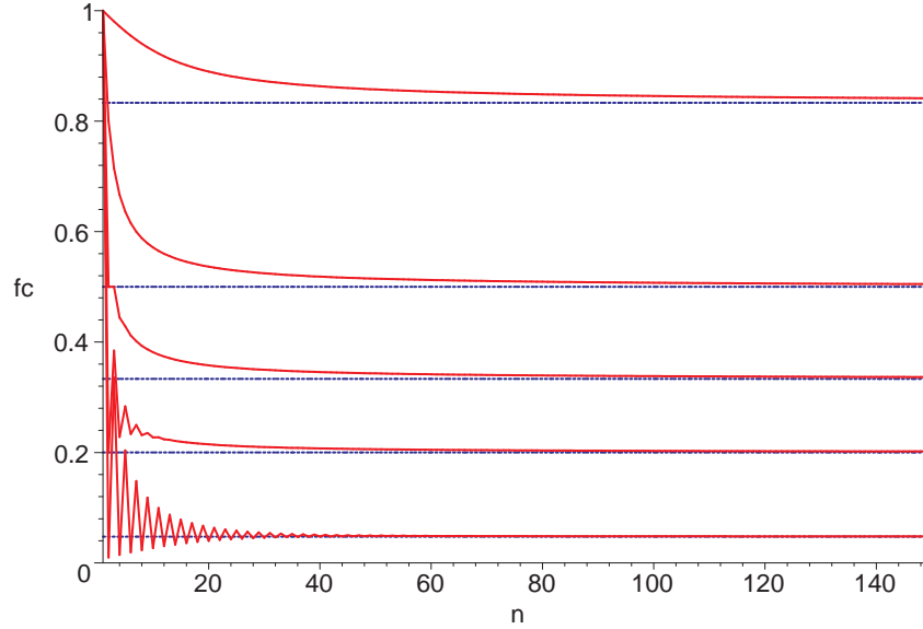
Figure 2: Convergence toward the asymptotic regimes (Dashed lines) of the proportions f_c (Solid lines) of unary nodes among \pi -weighted unary/binary trees of size n . Five values for the couple (\pi, f_c) are shown here (From top to bottom): (10, 5/6) , (2, 1/2) , (1, 1/3) , (1/2, 1/5) , and (1/10, 1/21) .
