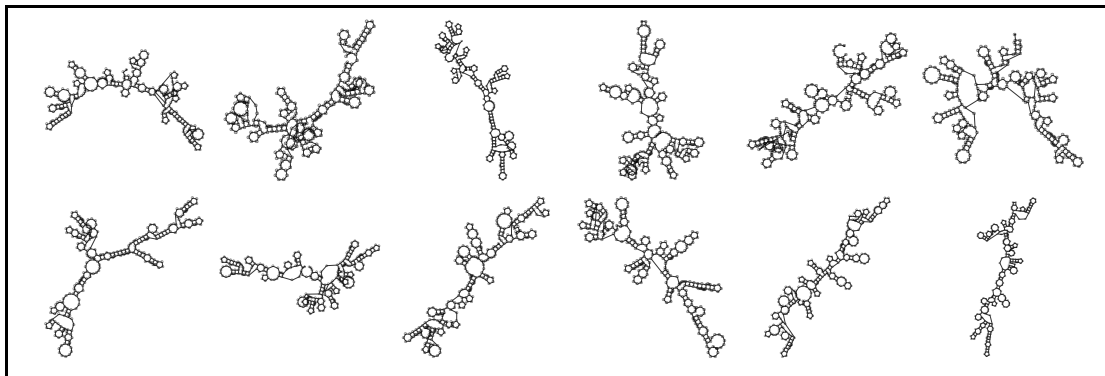
Uniform model \mathcal{M}_0
