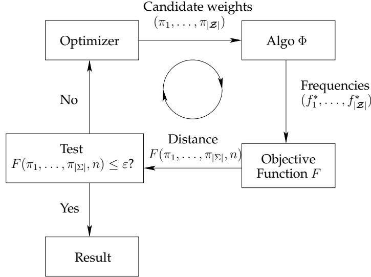
Figure 7: General principle of our heuristic approach to the problem of computing weights \pi that achieve targeted frequencies \mu .
