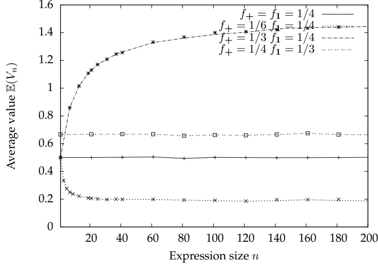
Figure 4: Average value of an arithmetic expression, computed by generating 100 000 random expression, for various sizes n and frequencies of symbols + and 1 .
