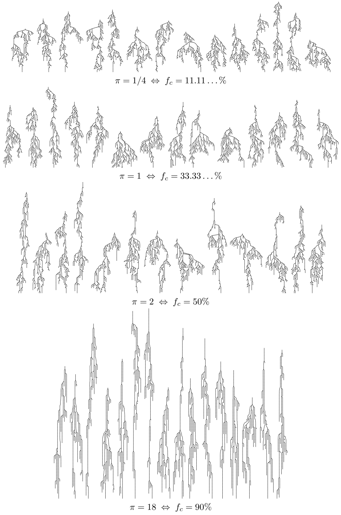
Figure 3: Unary-binary trees associated with weighted Motzkin words of size 500, for different values of \pi the weight of unary nodes.
