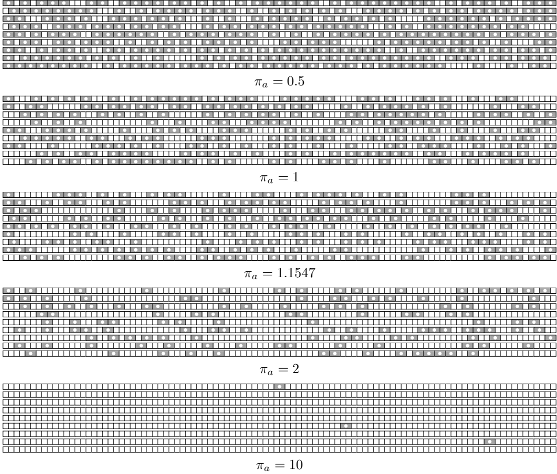
Figure 5: Sets of randomly generated Fibonacci words of length 100 for different values of \pi_a . White boxes: a 's; grey boxes: b 's
