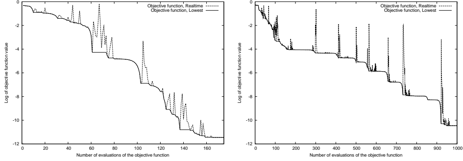
Figure 12: Minimization of the objective functions in the Helices (Left) and Loops (Right) models. A logarithmic scale is used for the value of the objective function (Y-axis).
