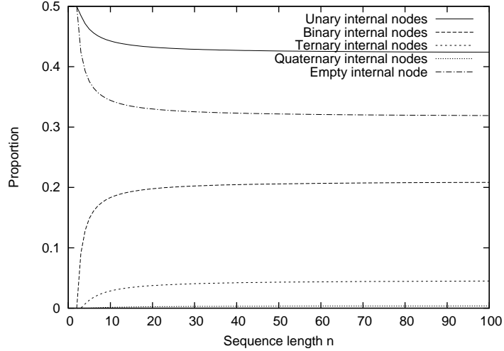
Figure 8: Evolution of the node degree distribution for trees of increasing size in the uniform model. The asymptotic proportions of nodes of degree (0, 1, 2, 3, 4) are respectively (81/256, 27/64, 27/128, 3/64, 1/256) .
