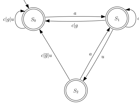
Figure 6: A finite state automaton recognizing the language generated by the grammar.
