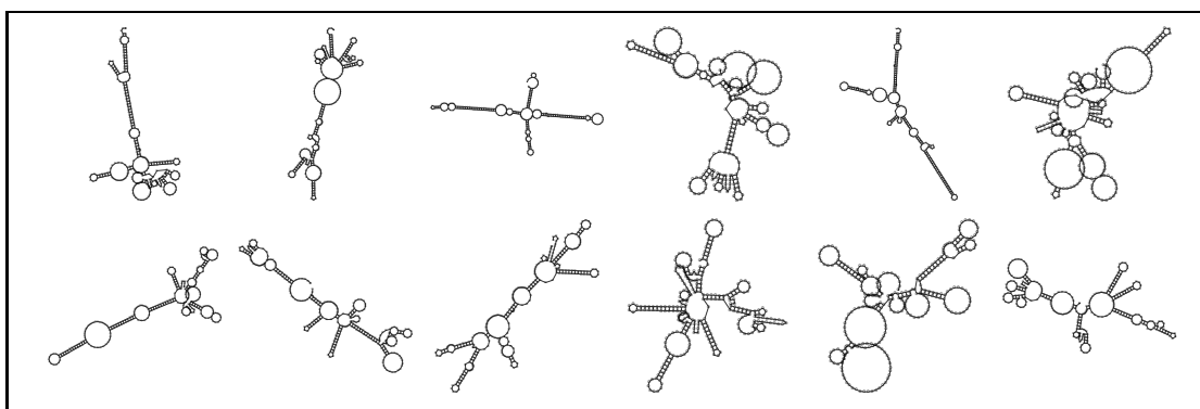
Helices model \mathcal{M}_H : Constraints on expected number and length for hairpins.
